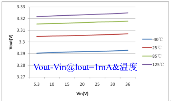
Line Regulation Iout=1mA
