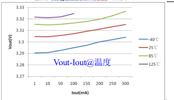
Load Regulation
