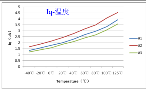
DC Supply Quiescent Current
