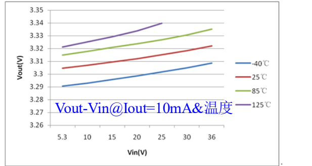
Line Regulation Iout=10mA
