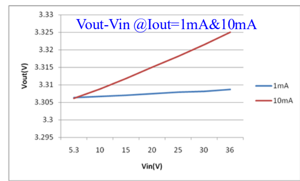
Line Regulation
